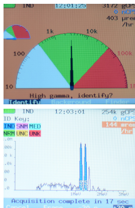
SAM940-SIM-Nal-P simulates the display of alarms and identification of nuclear isotopes
